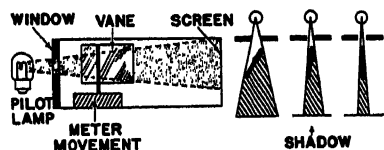
Shadow tuning indicator.
